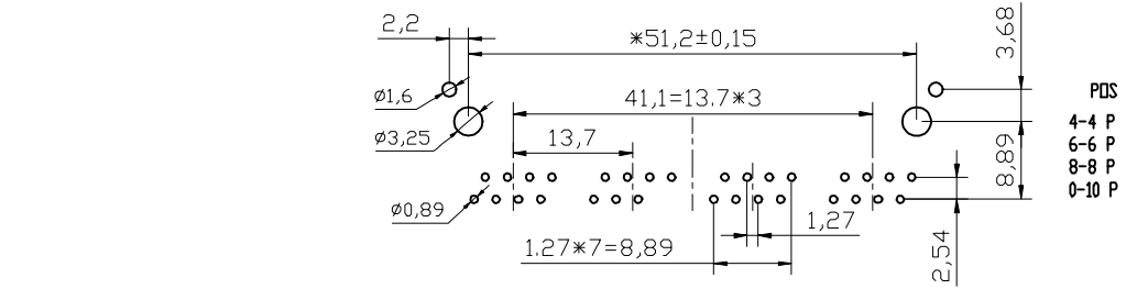
PC Board Layout Component Side Shown
