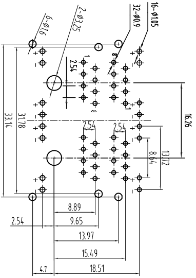
PC Board Layout Component Side Shown
