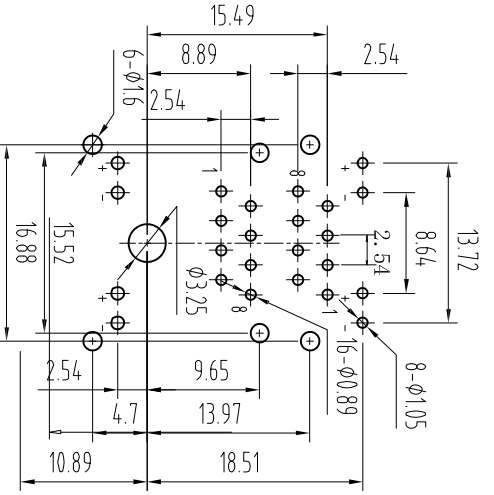
PC Board Side Layout Component Side Shown
