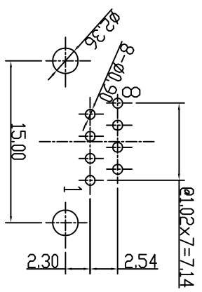
PC BOARD LAYOUT THICKNESS=1.6MM
