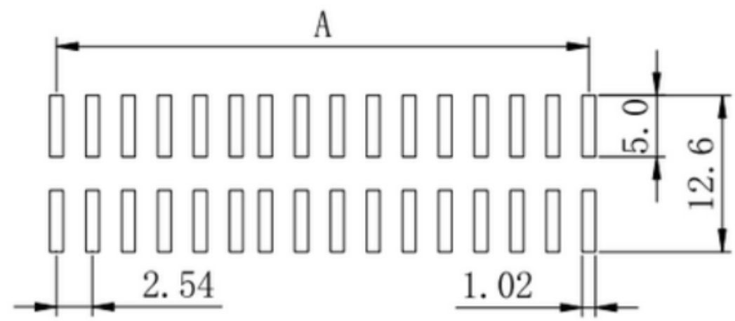
PCB LAYOUT
