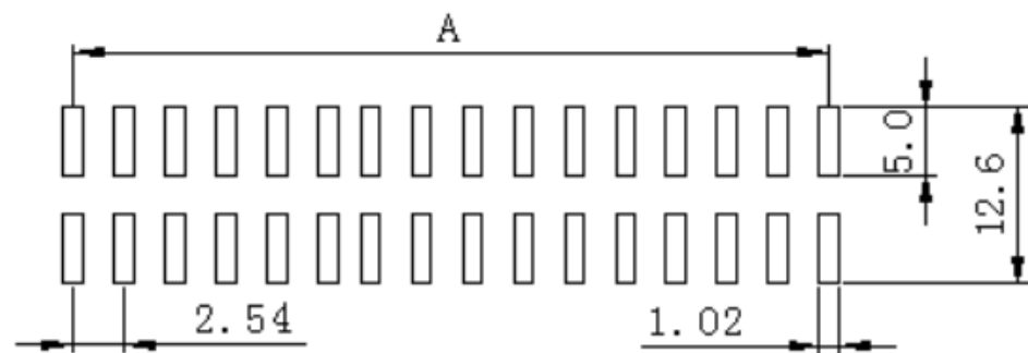
PCB LAYOUT
