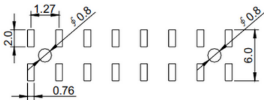
PCB LAYOUT
